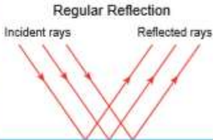
Figure 3.8 Regular reflection
