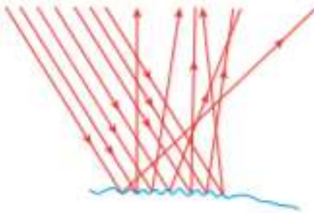
Figure 3.8 Irregular reflection
