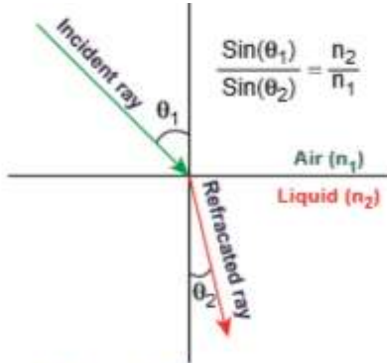
Figure 3.12 Snell's Law
